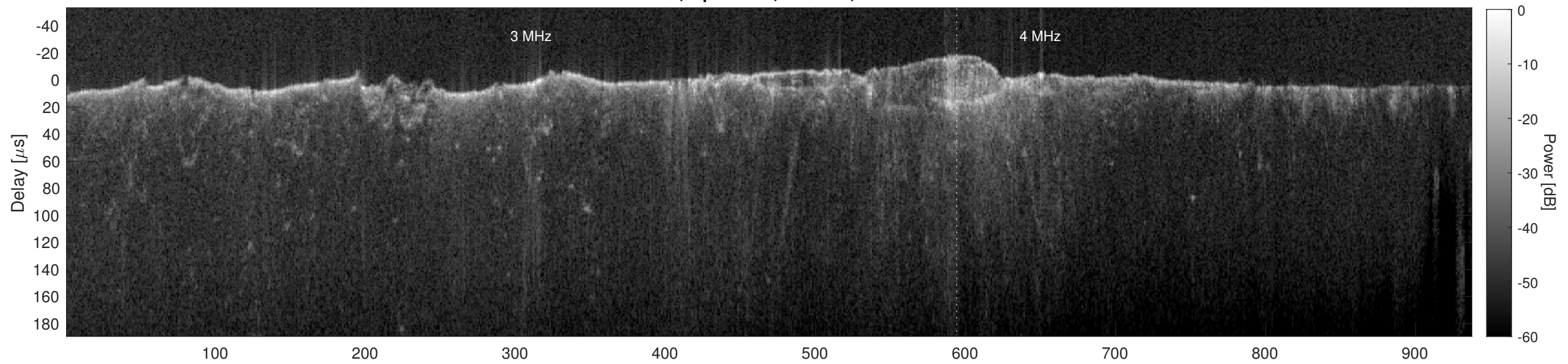
Orbit 8729, Cluttergram
