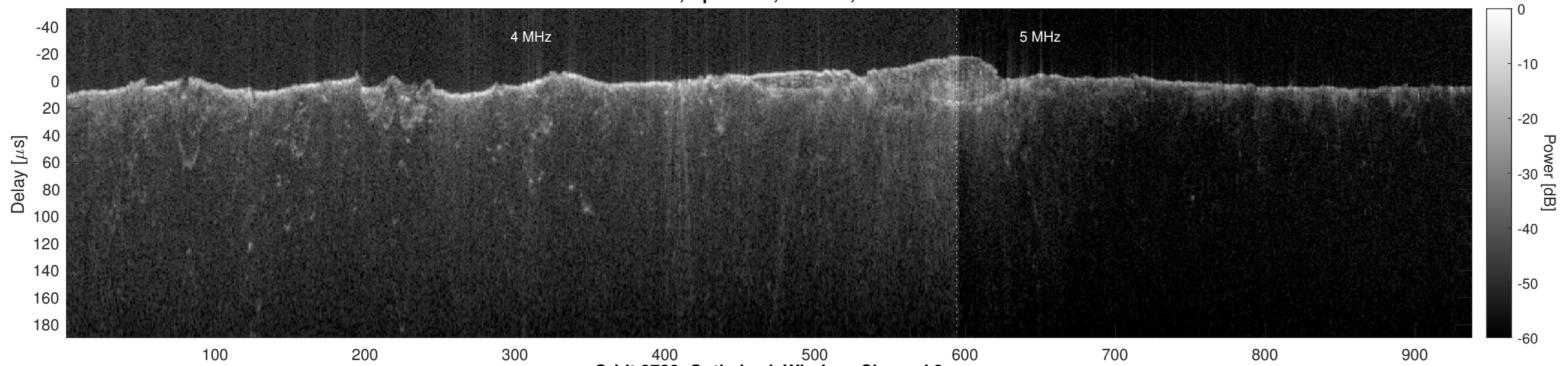
Orbit 8729, Optimized, Window, Channel 2
