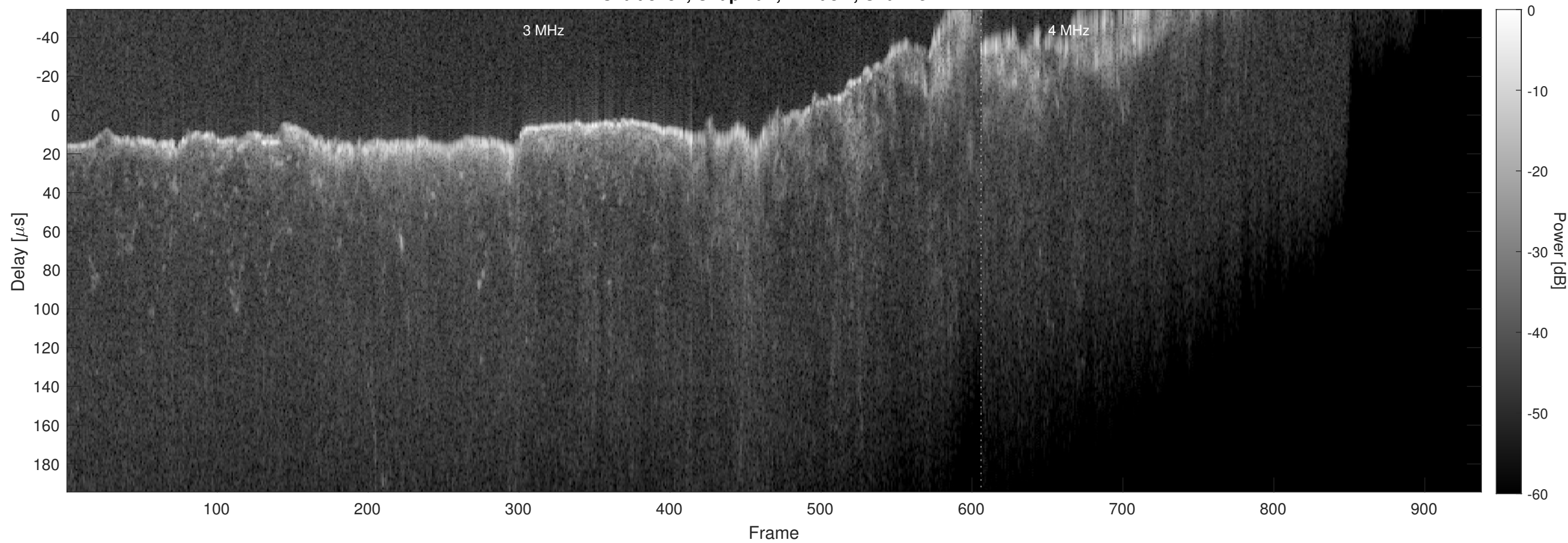
Orbit 8731, Chapman, Window, Channel 2
