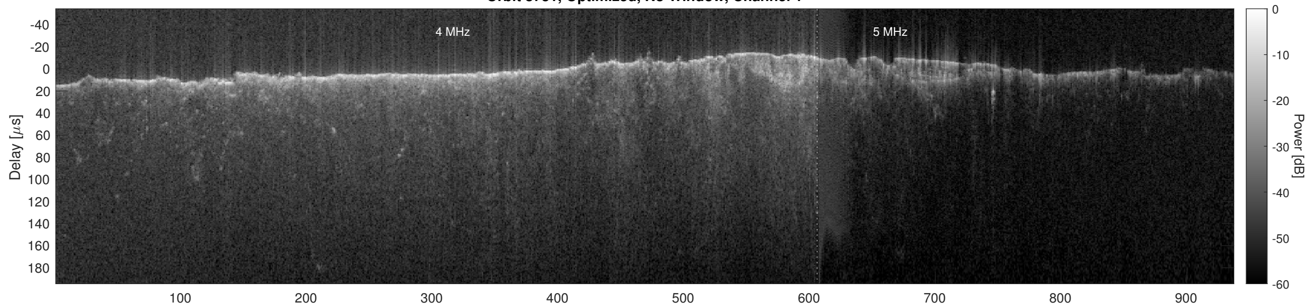
Orbit 8731, Optimized, No Window, Channel 2
