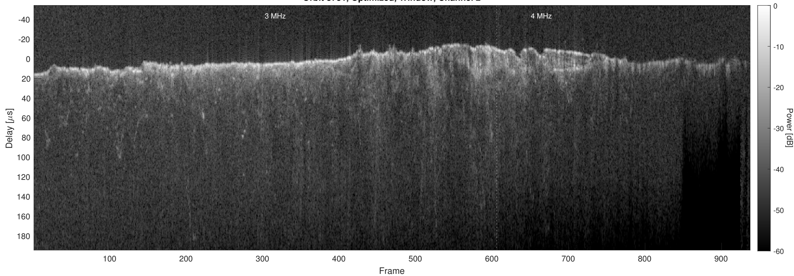
Orbit 8731, Optimized, Window, Channel 2
