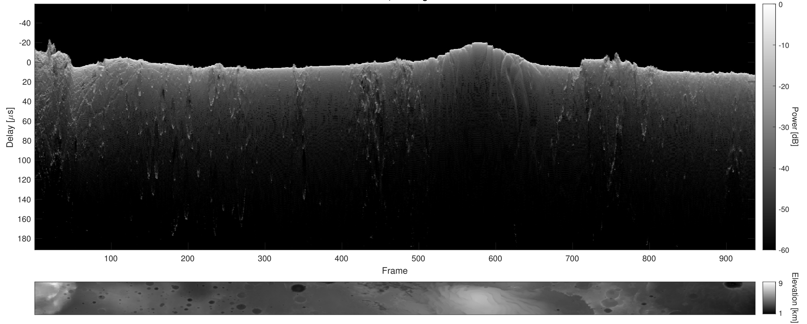
Orbit 8732, Cluttergram
