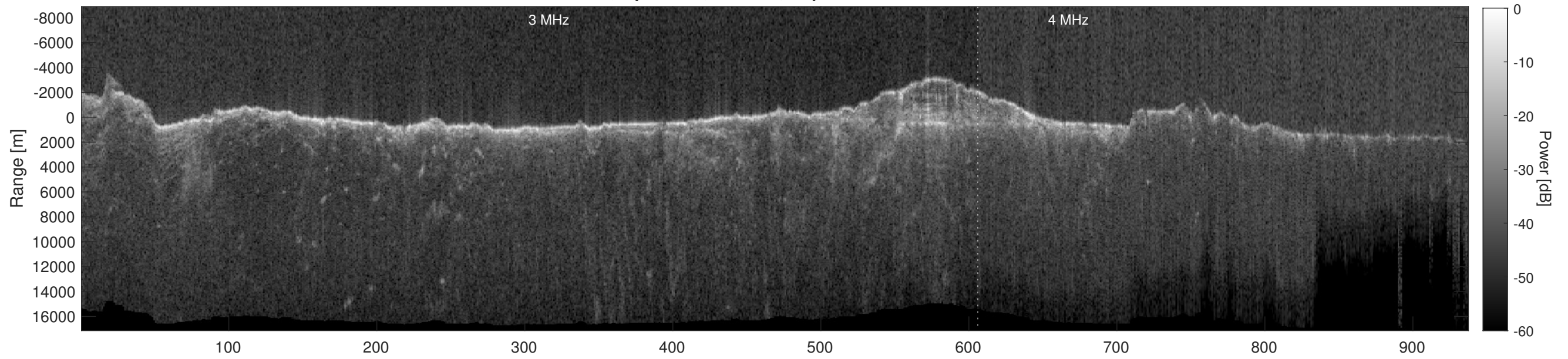
Orbit 8732, Depth-Corrected Cluttergram
