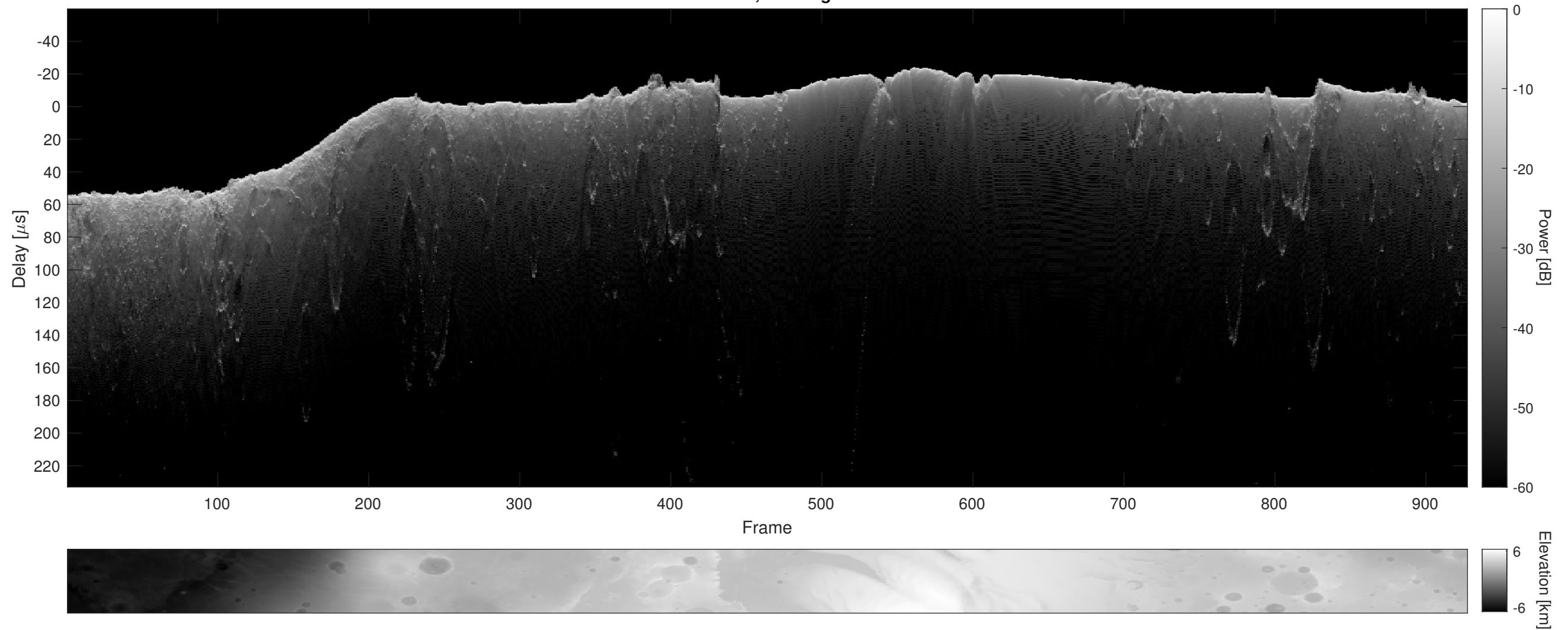
Orbit 8734, Cluttergram
