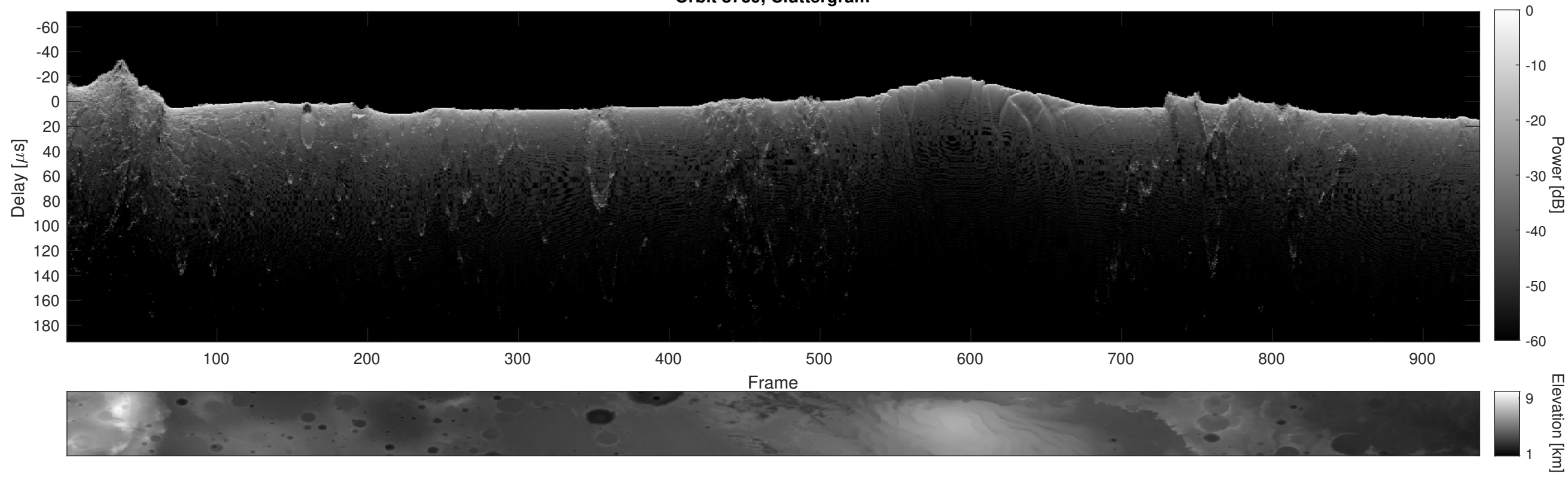
Orbit 8739, Cluttergram
