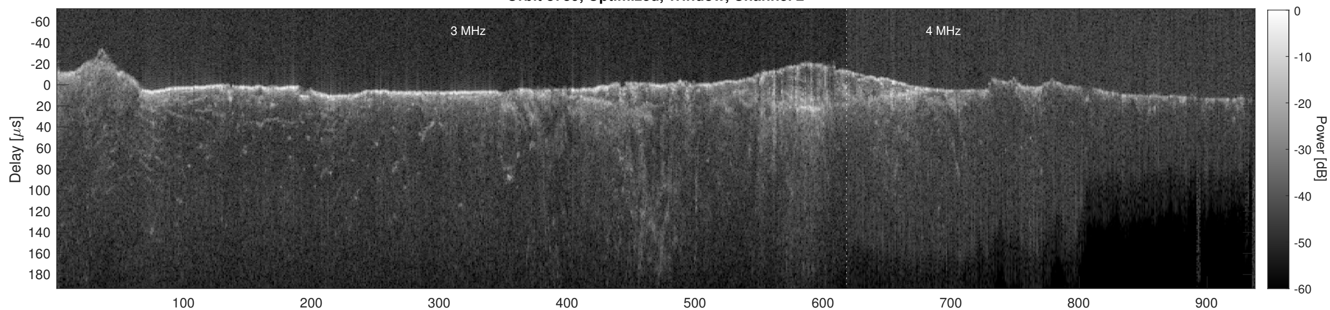
Orbit 8739, Cluttergram
