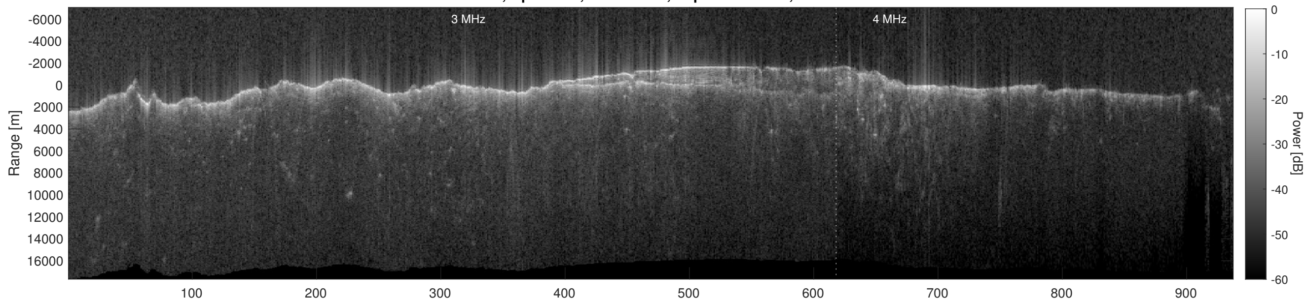
Orbit 8740, Depth-Corrected Cluttergram
