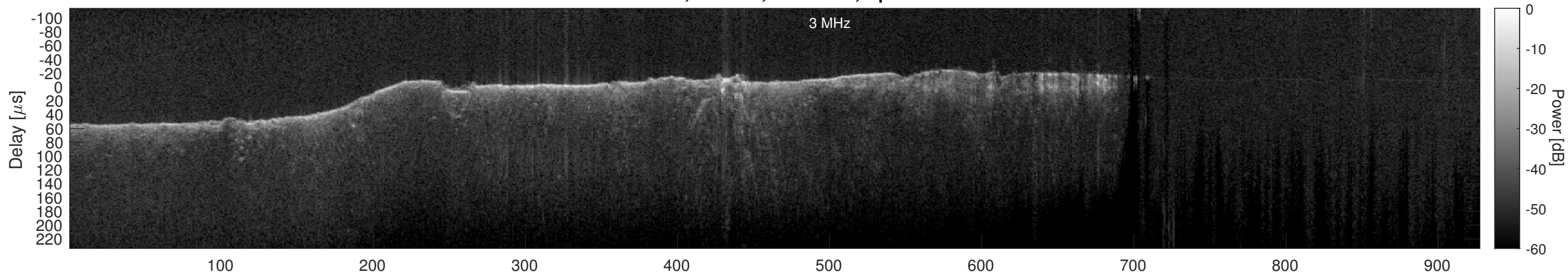
Orbit 8741, Cluttergram
