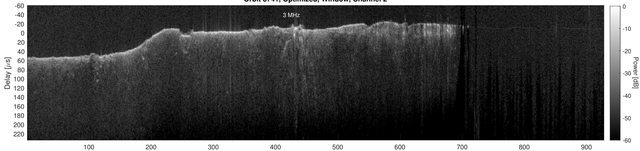
Orbit 8741, Cluttergram
