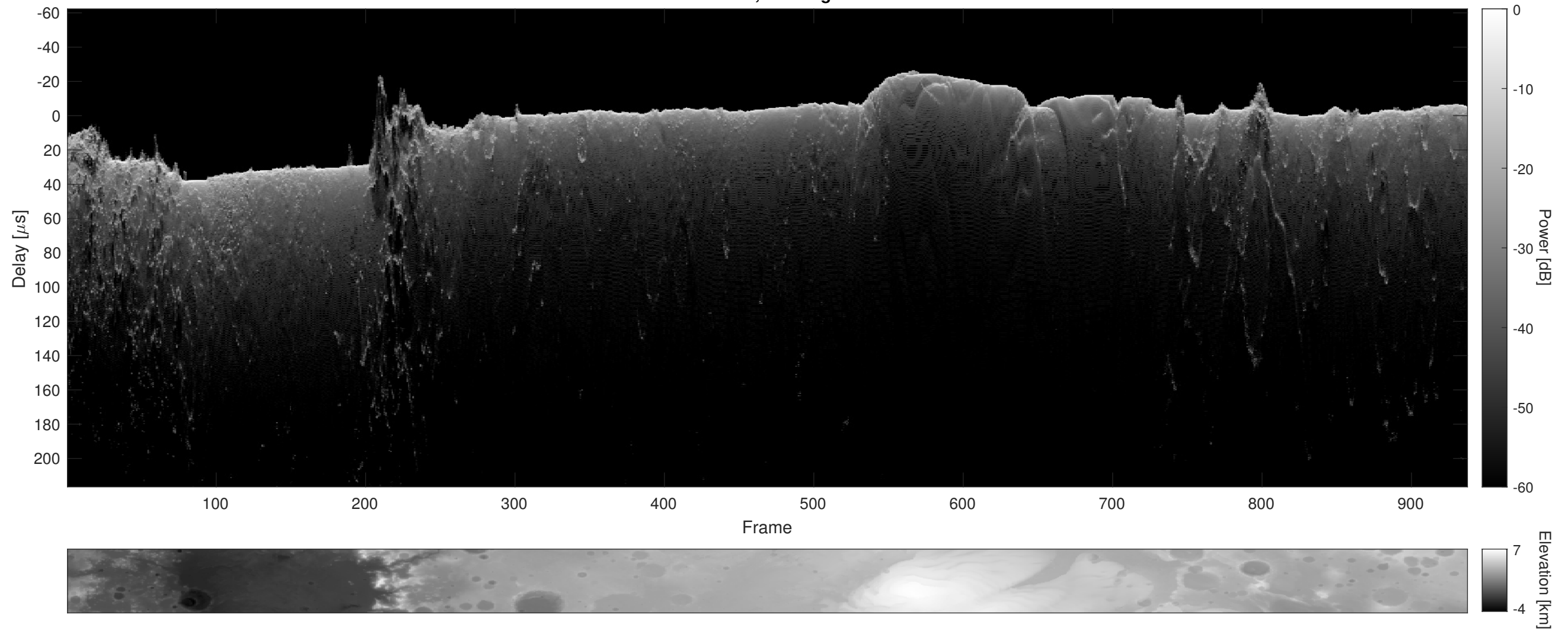
Orbit 8742, Cluttergram
