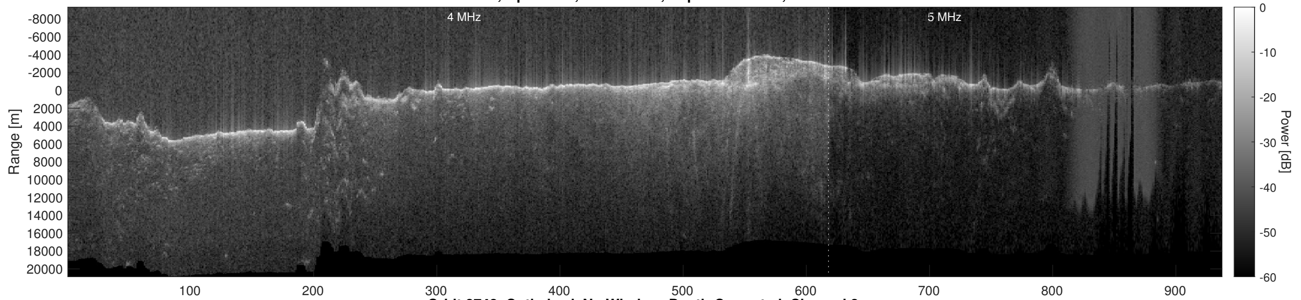
Orbit 8742, Optimized, No Window, Depth-Corrected, Channel 2
