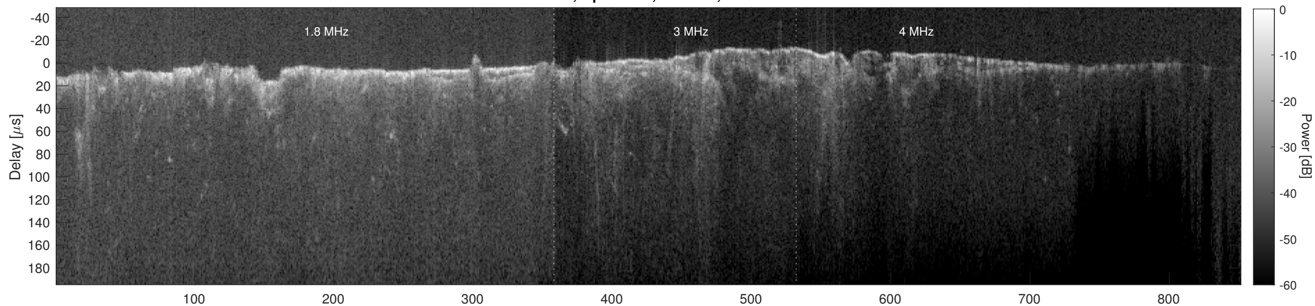
Orbit 8745, Cluttergram
