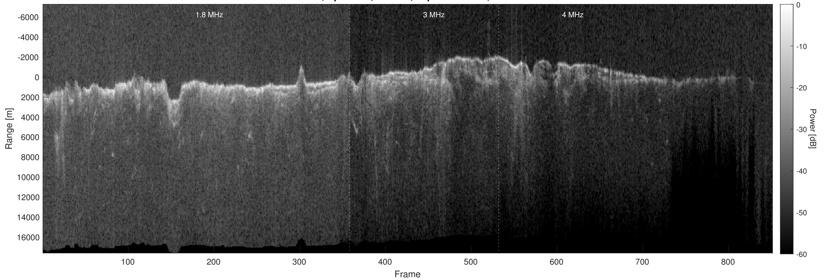
Orbit 8745, Optimized, Window, Depth-Corrected, Channel 2
