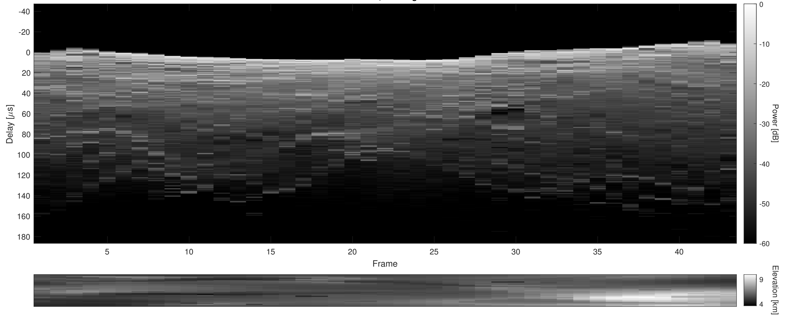
Orbit 8746, Cluttergram
