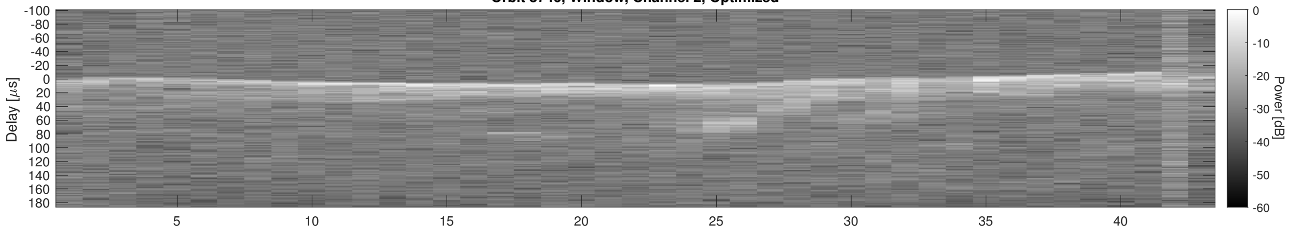
Orbit 8746, Cluttergram
