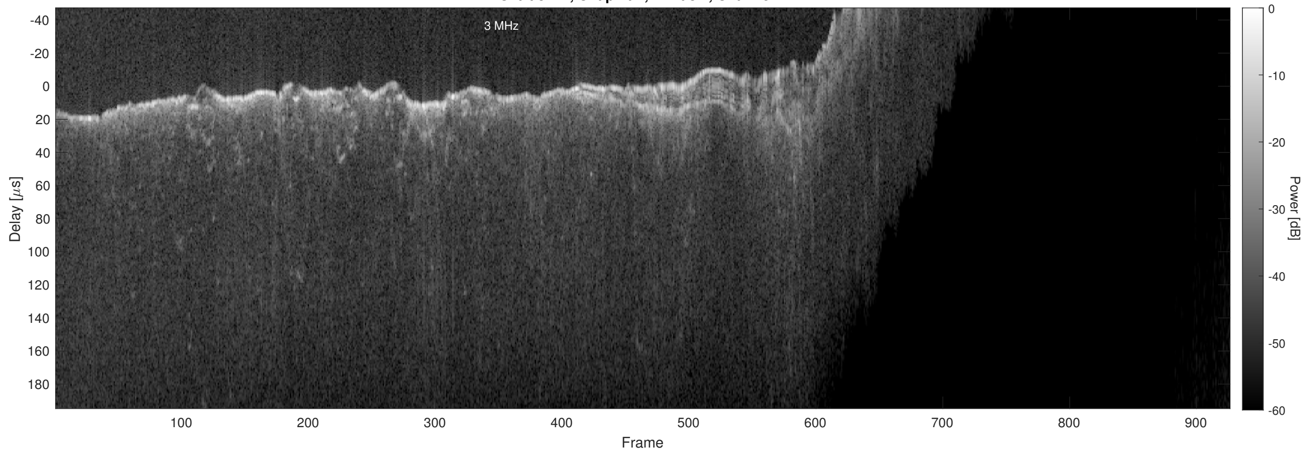
Orbit 8747, Chapman, Window, Channel 2
