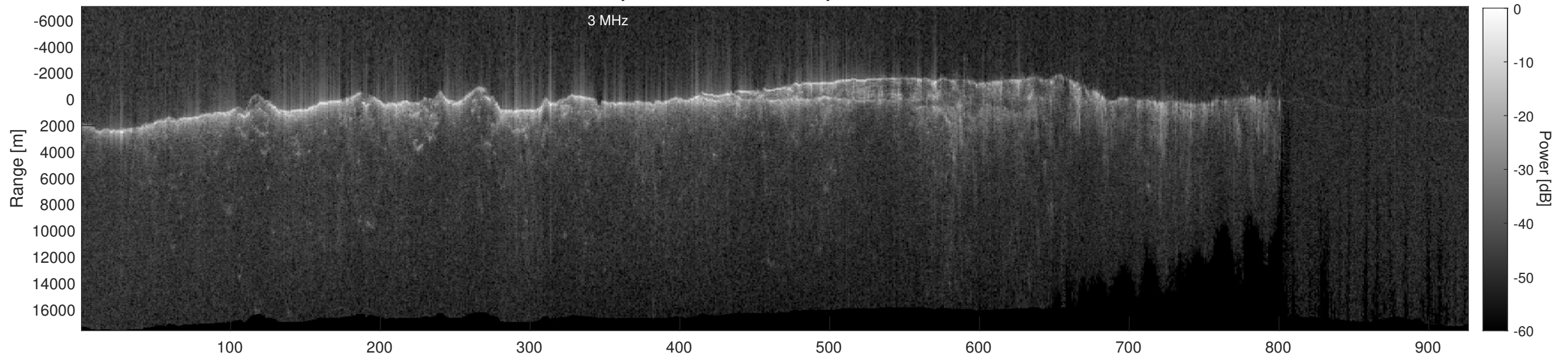
Orbit 8747, Depth-Corrected Cluttergram
