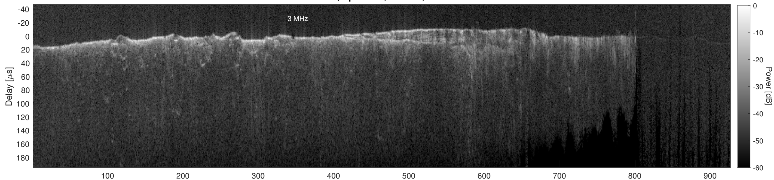
Orbit 8747, Cluttergram
