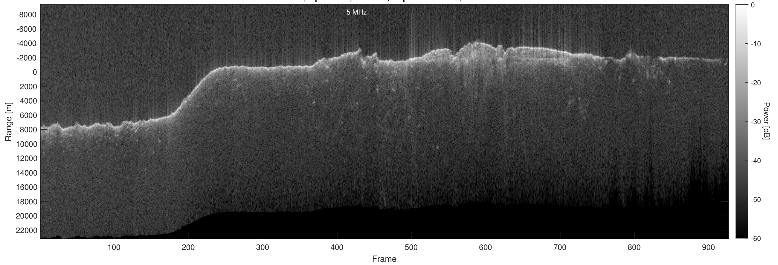
Orbit 8748, Optimized, Window, Depth-Corrected, Channel 2
