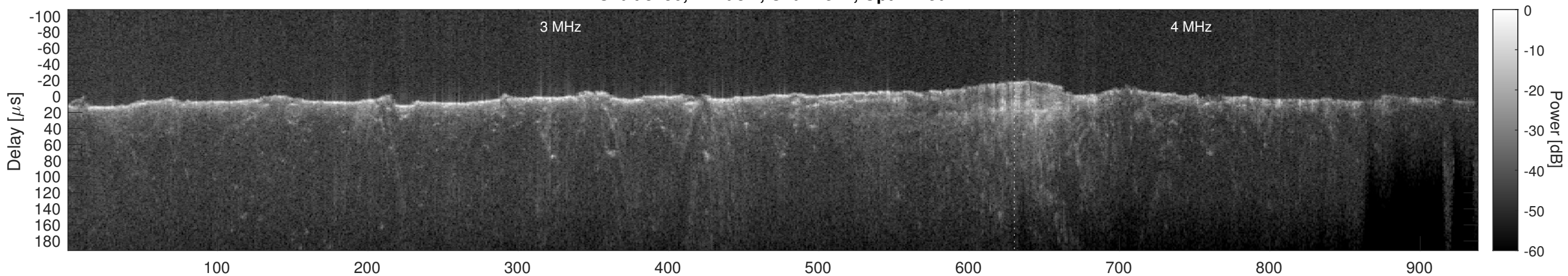
Orbit 8750, Cluttergram
