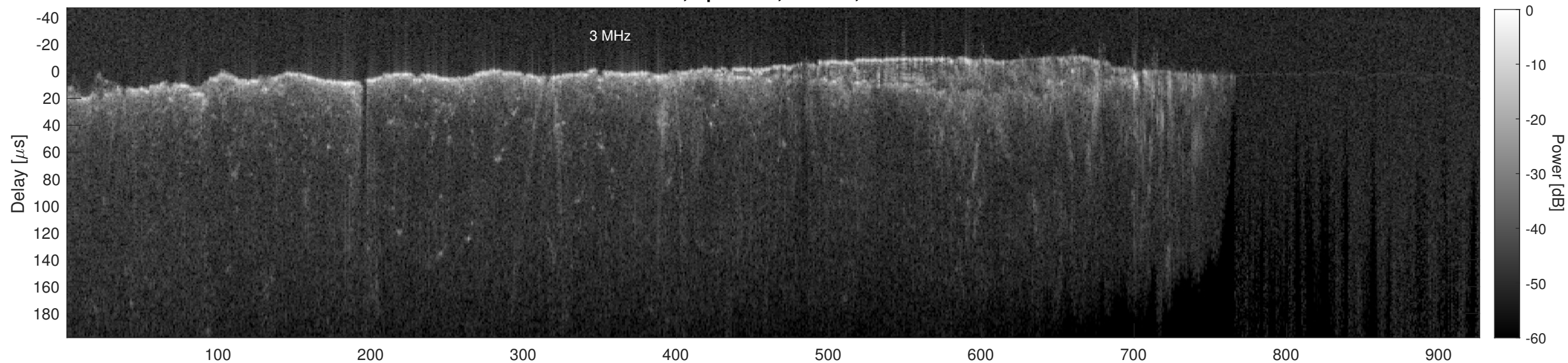
Orbit 8754, Cluttergram
