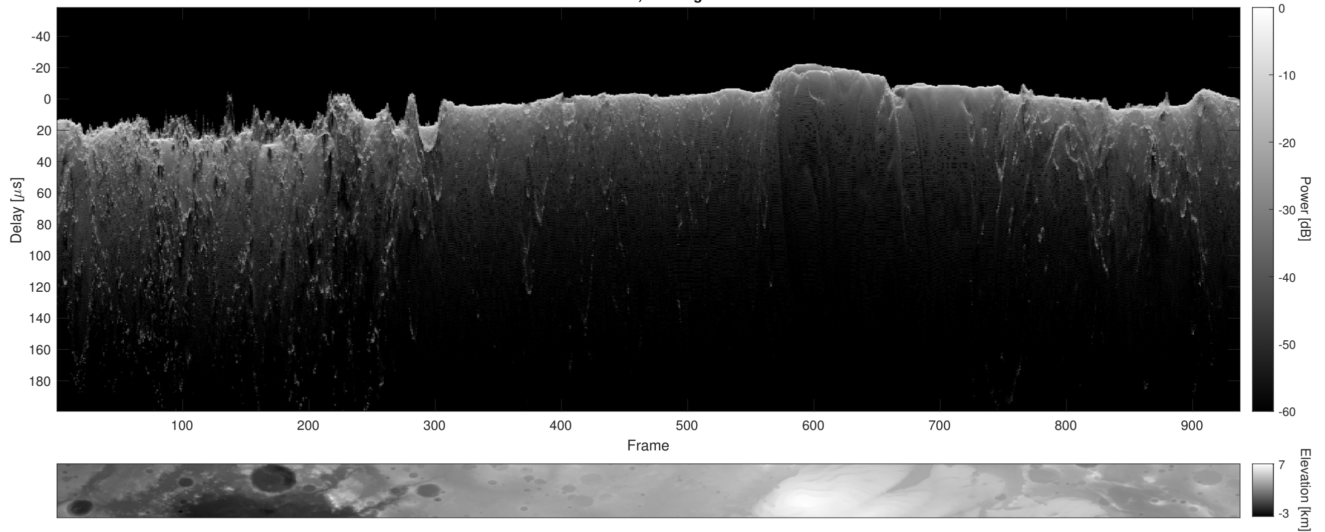
Orbit 8756, Cluttergram
