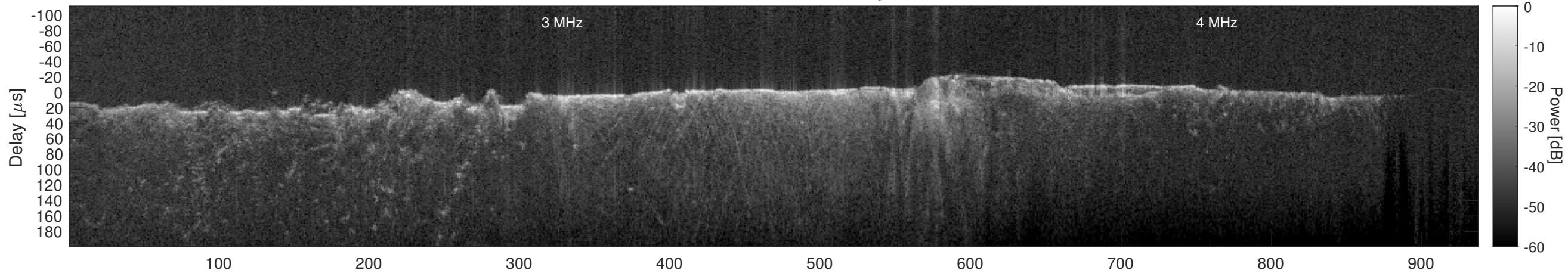
Orbit 8756, Cluttergram
