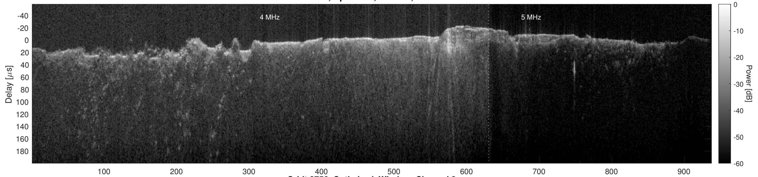
Orbit 8756, Optimized, Window, Channel 2
