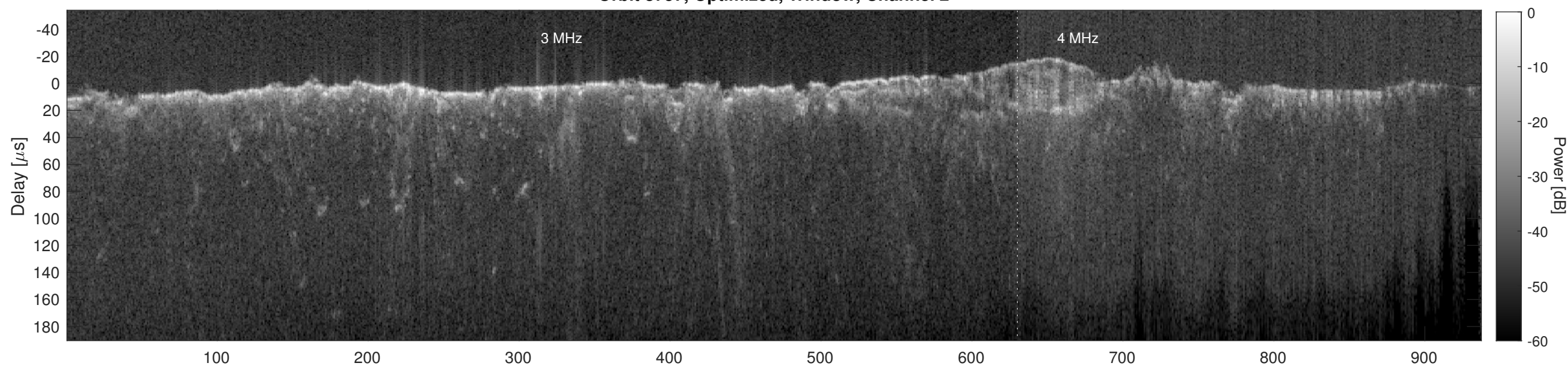
Orbit 8757, Cluttergram
