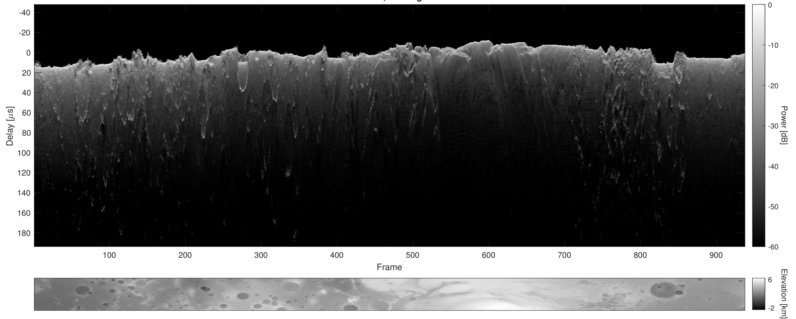
Orbit 8758, Cluttergram
