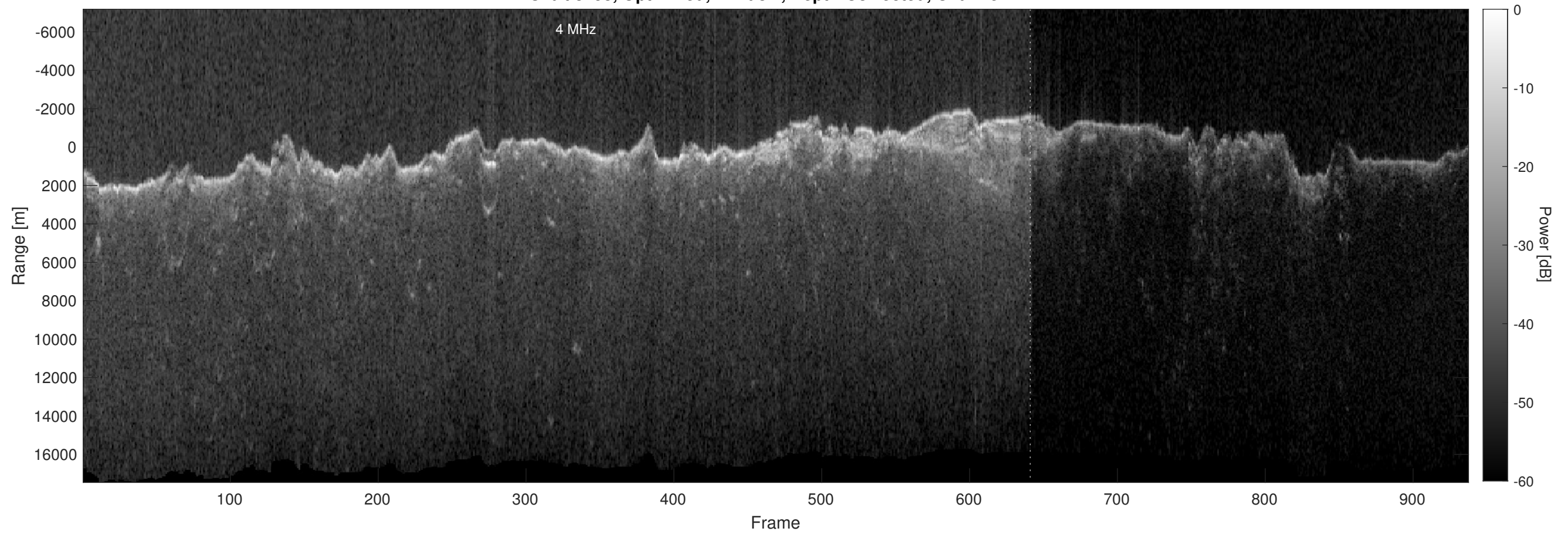
Orbit 8758, Optimized, Window, Depth-Corrected, Channel 2
