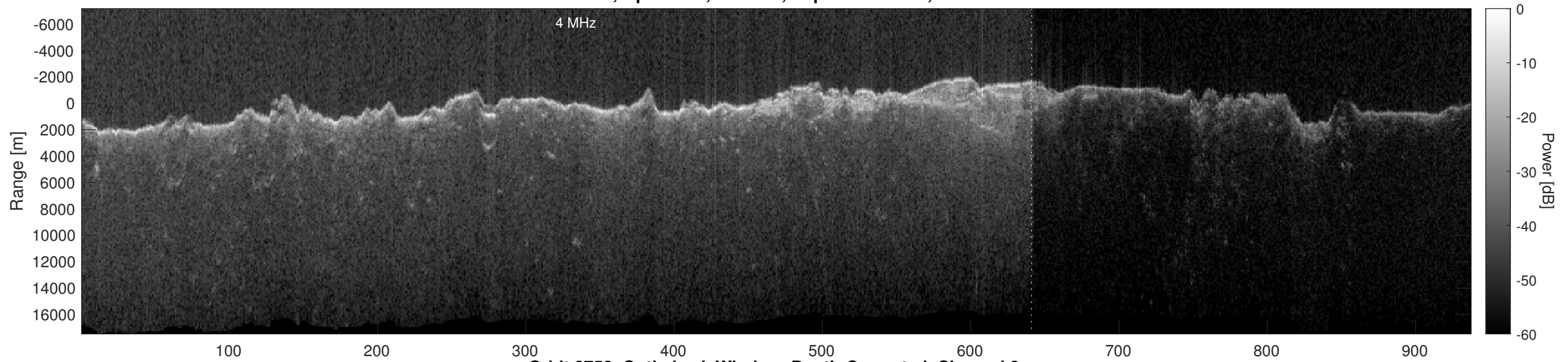
Orbit 8758, Optimized, Window, Depth-Corrected, Channel 2
