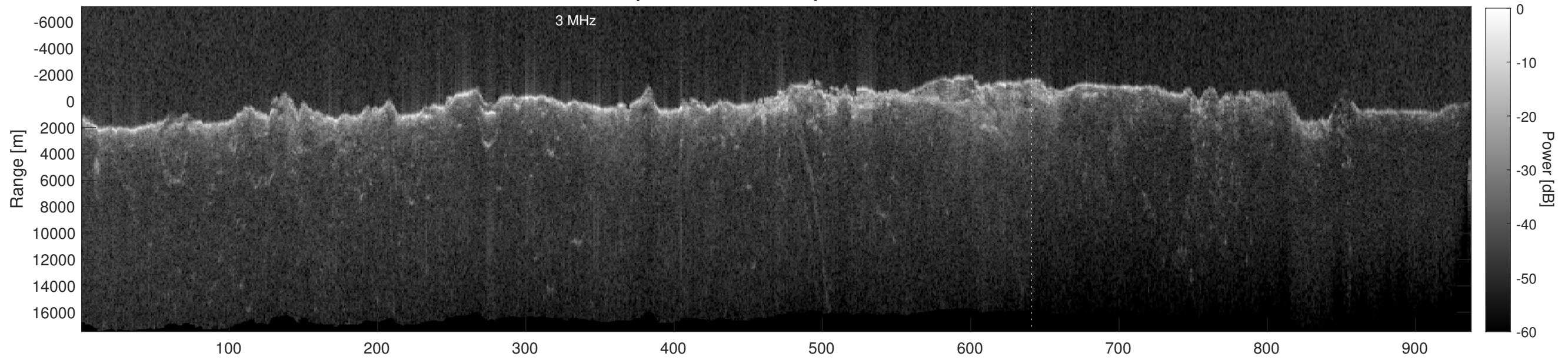
Orbit 8758, Depth-Corrected Cluttergram
