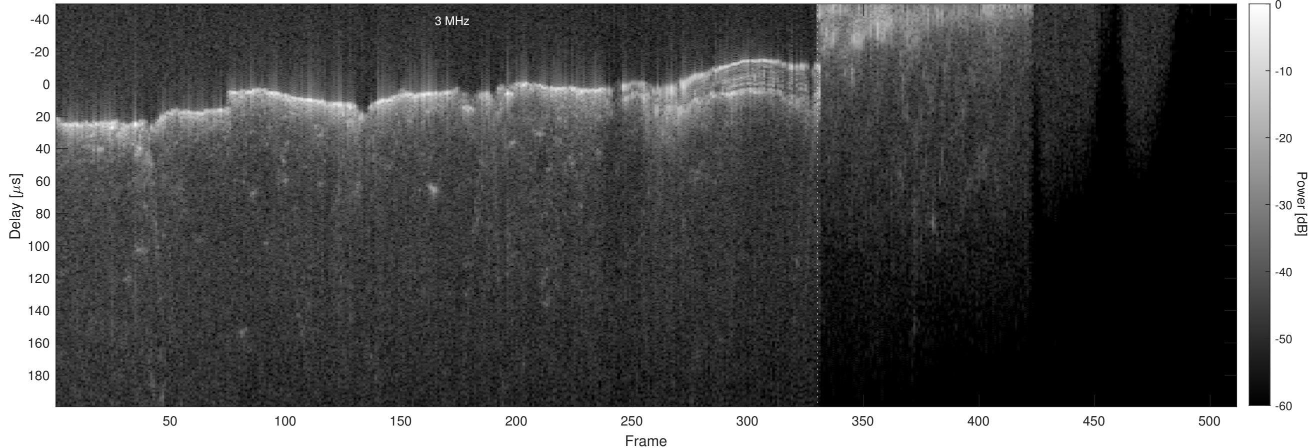
Orbit 8761, Chapman, No Window, Channel 2
