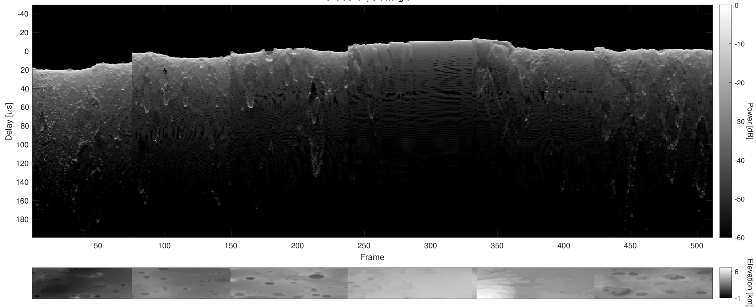
Orbit 8761, Cluttergram
