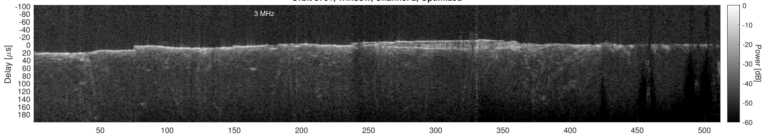
Orbit 8761, Cluttergram
