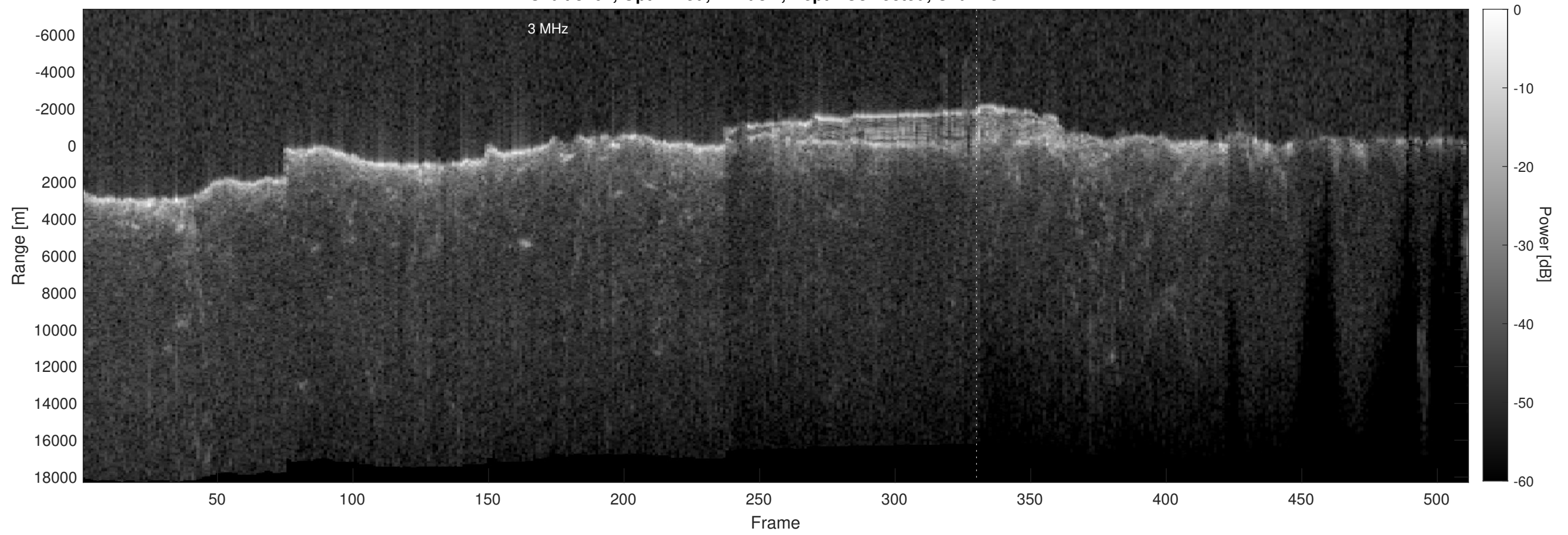
Orbit 8761, Optimized, Window, Depth-Corrected, Channel 2
