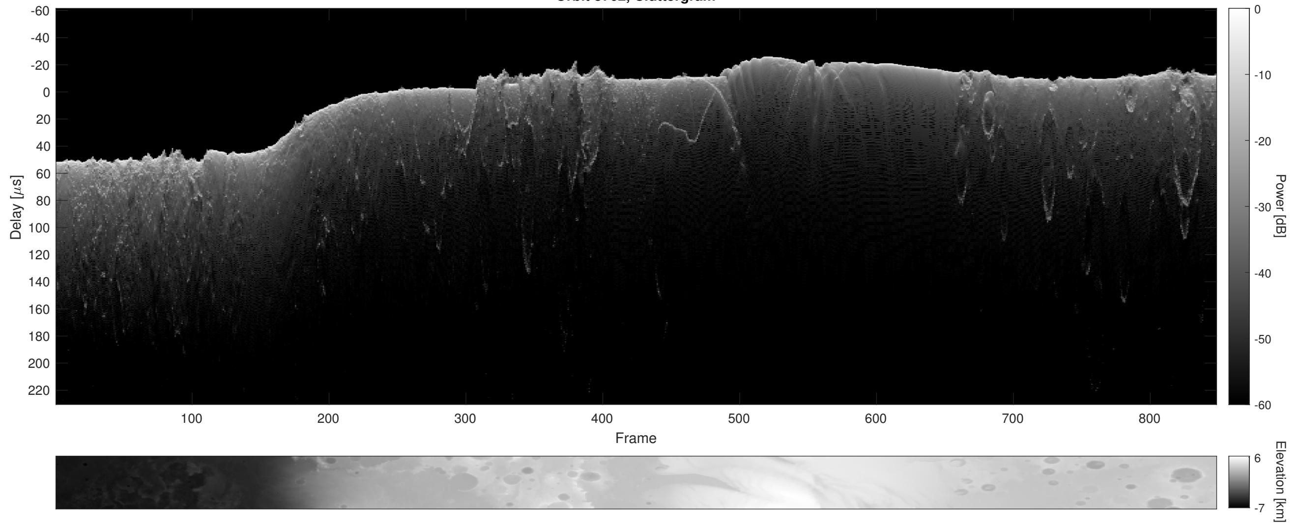
Orbit 8762, Cluttergram
