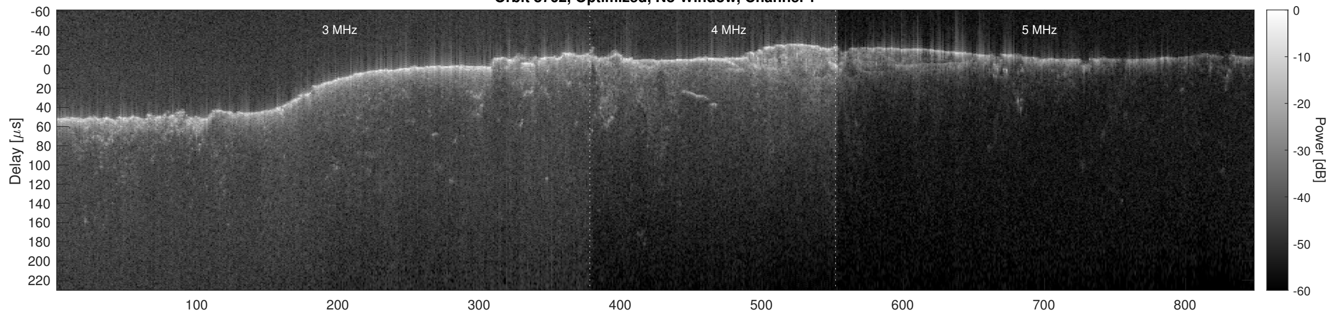
Orbit 8762, Optimized, No Window, Channel 2
