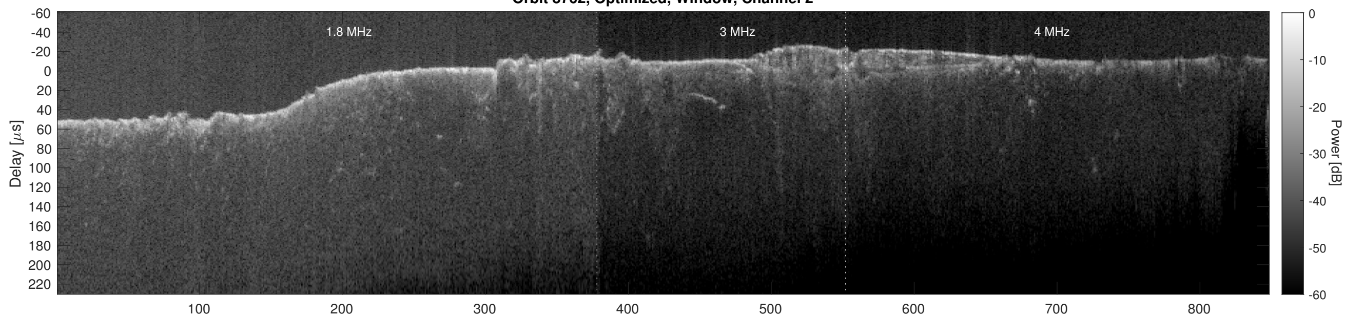
Orbit 8762, Cluttergram
