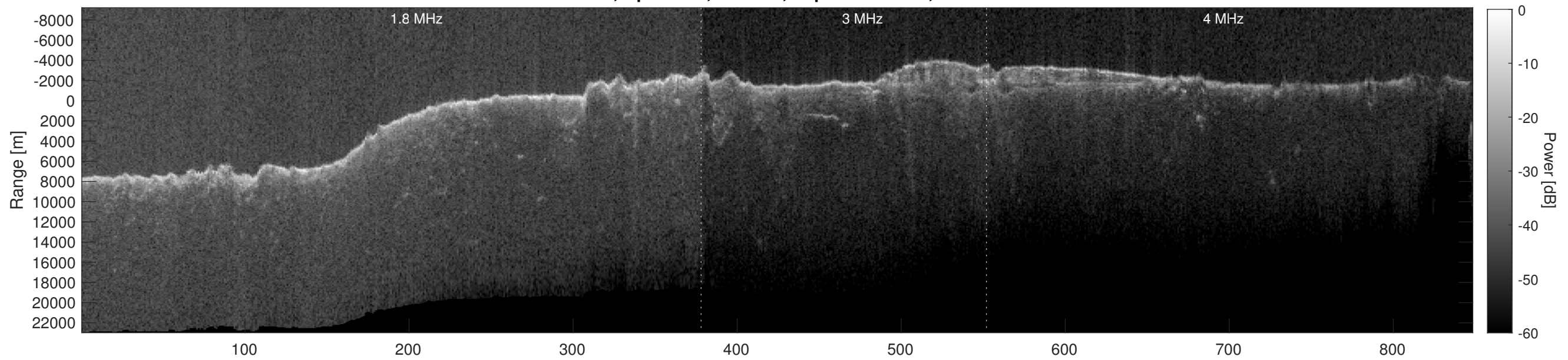
Orbit 8762, Depth-Corrected Cluttergram
