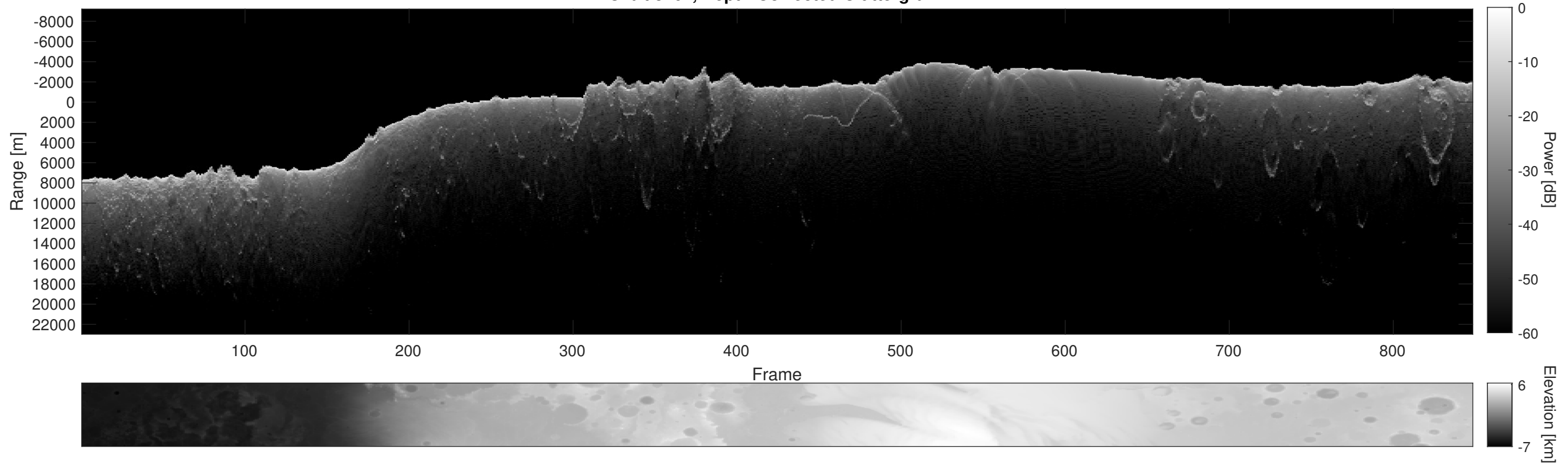
Orbit 8762, Depth-Corrected Cluttergram
