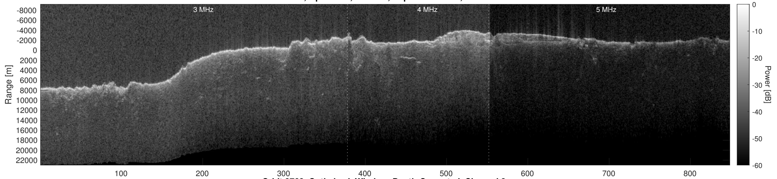
Orbit 8762, Optimized, Window, Depth-Corrected, Channel 2
