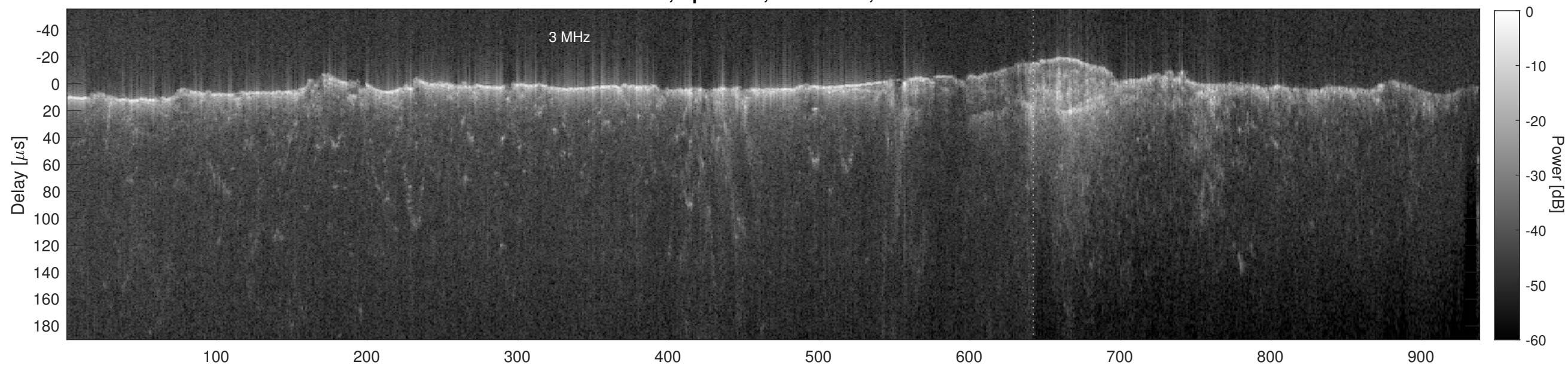
Orbit 8764, Cluttergram
