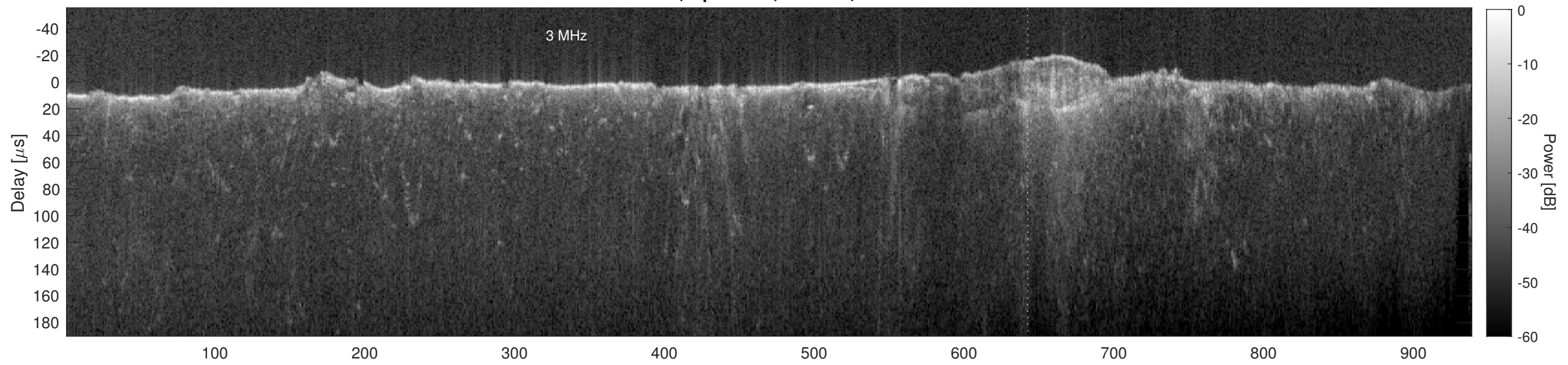
Orbit 8764, Cluttergram
