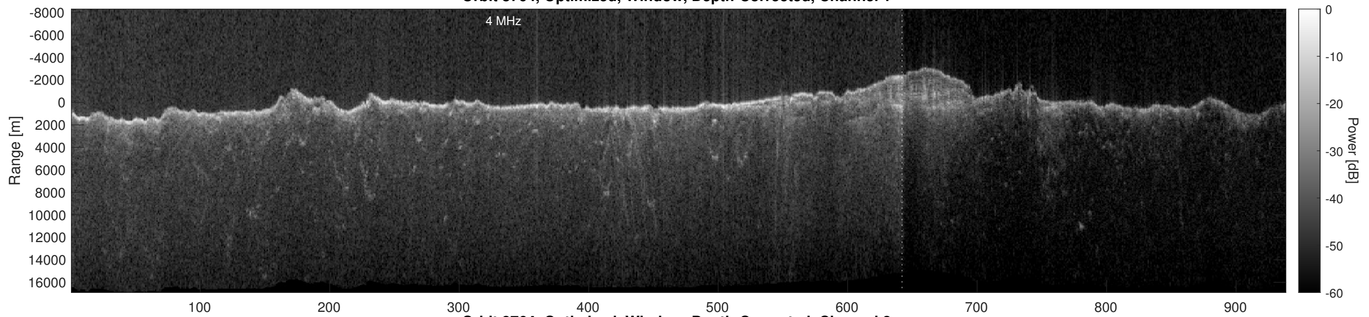
Orbit 8764, Optimized, Window, Depth-Corrected, Channel 2
