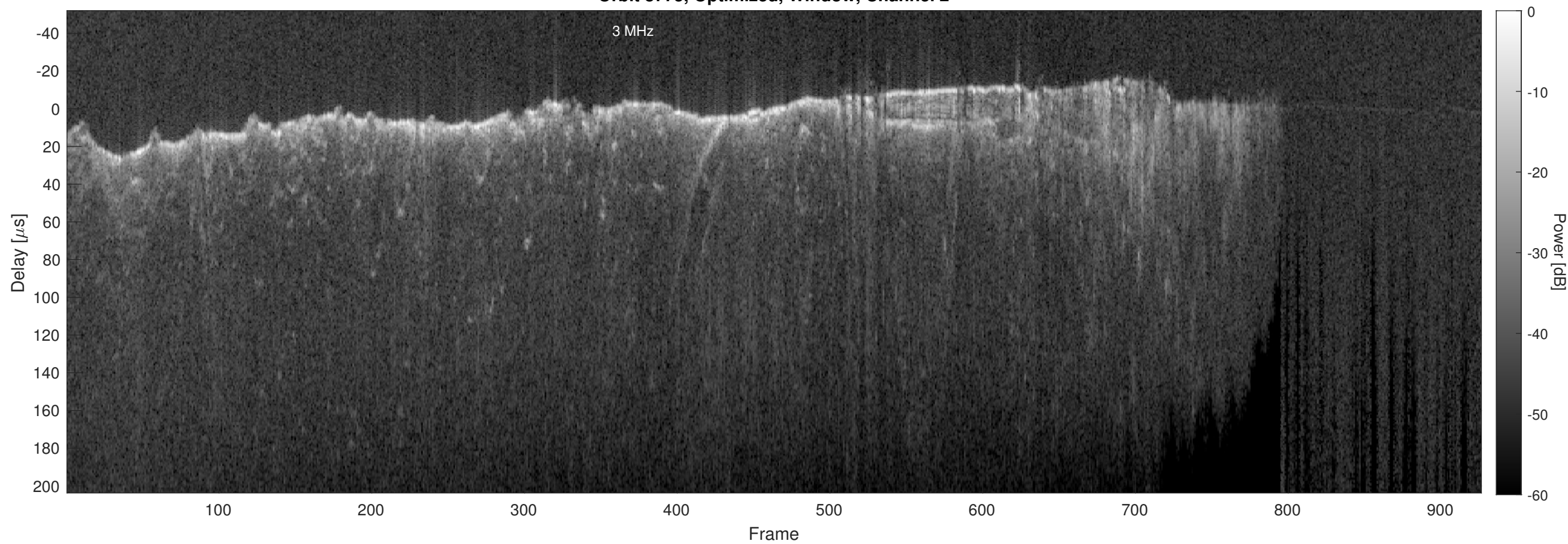
Orbit 8775, Optimized, Window, Channel 2
