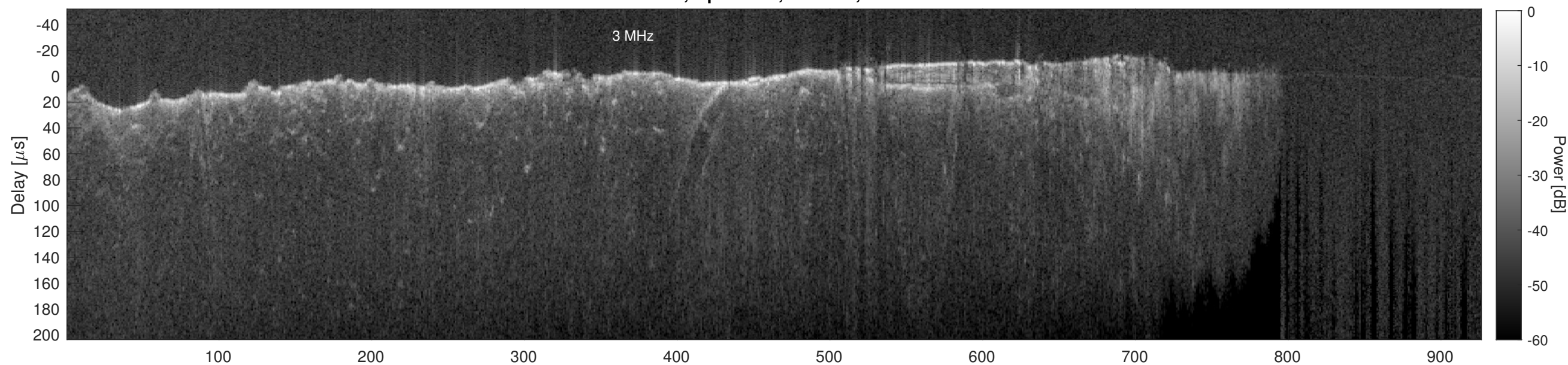
Orbit 8775, Cluttergram
