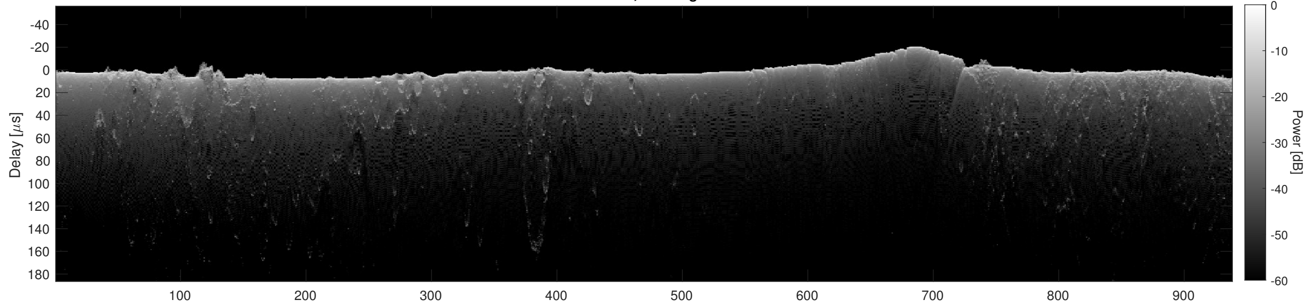
Orbit 8778, Cluttergram
