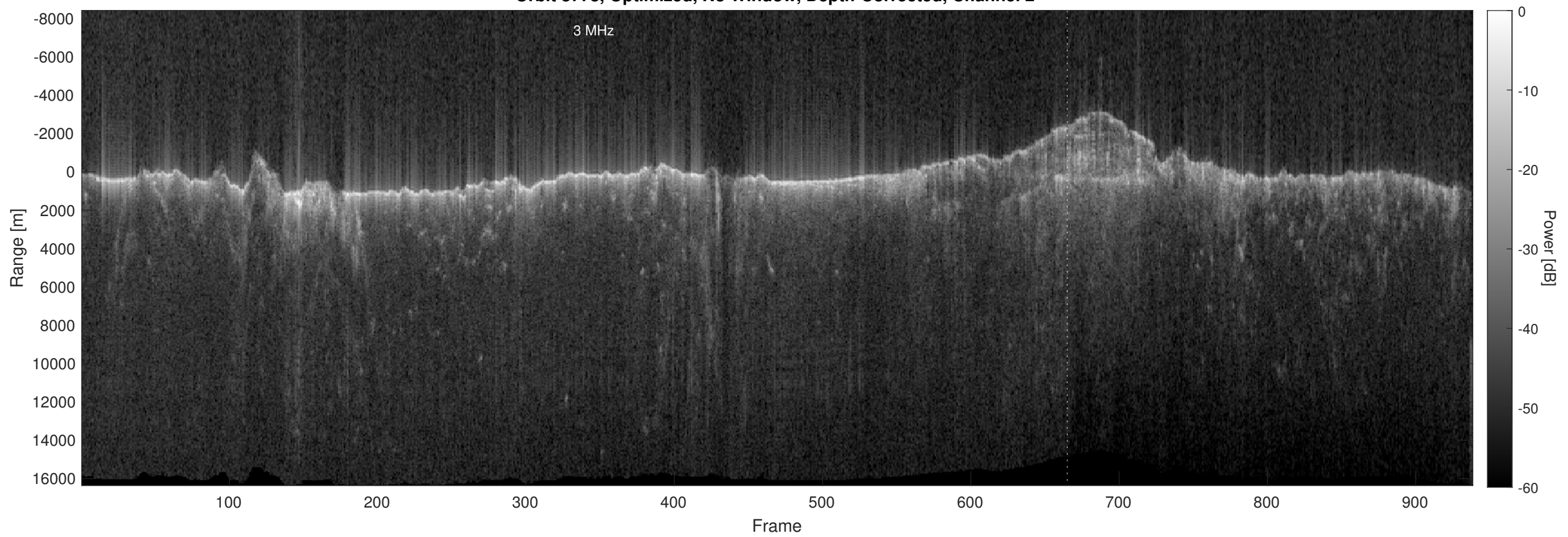
Orbit 8778, Optimized, No Window, Depth-Corrected, Channel 2
