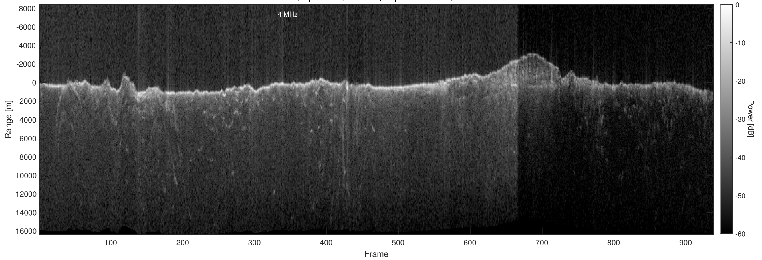
Orbit 8778, Optimized, Window, Depth-Corrected, Channel 2
