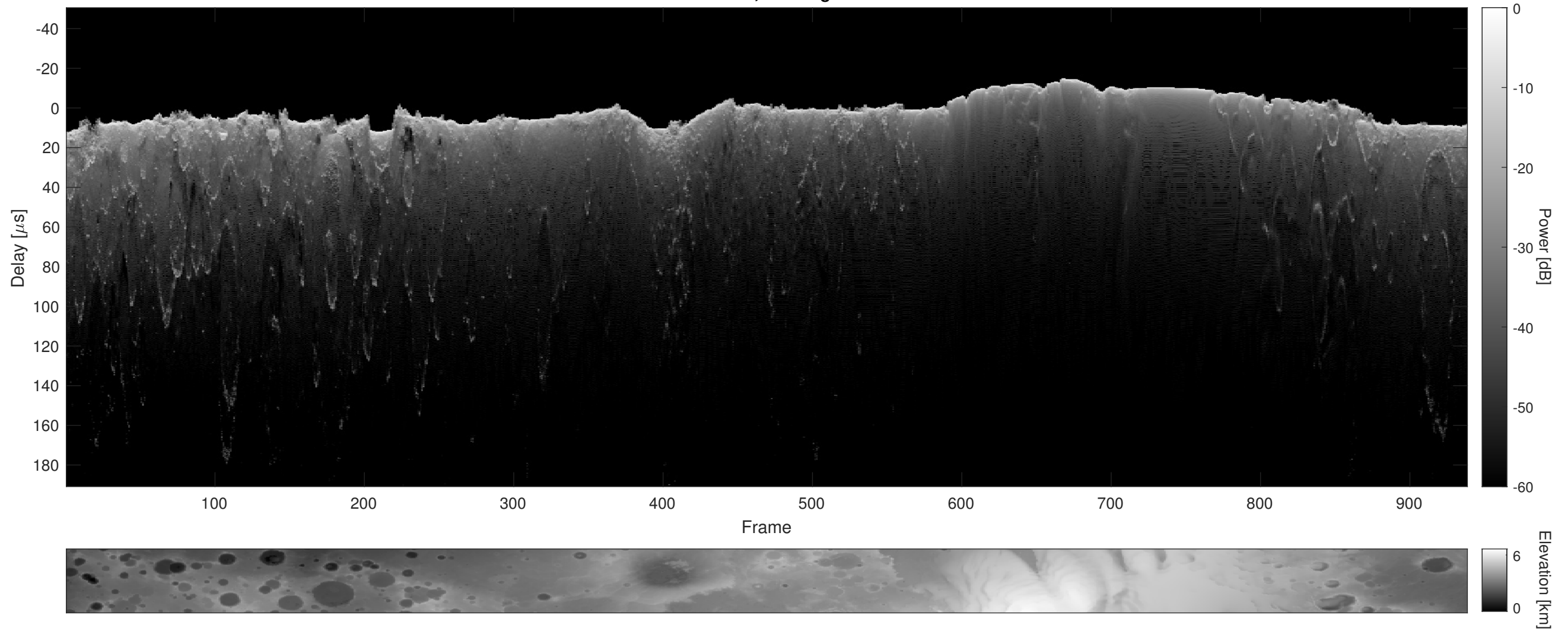
Orbit 8780, Cluttergram
