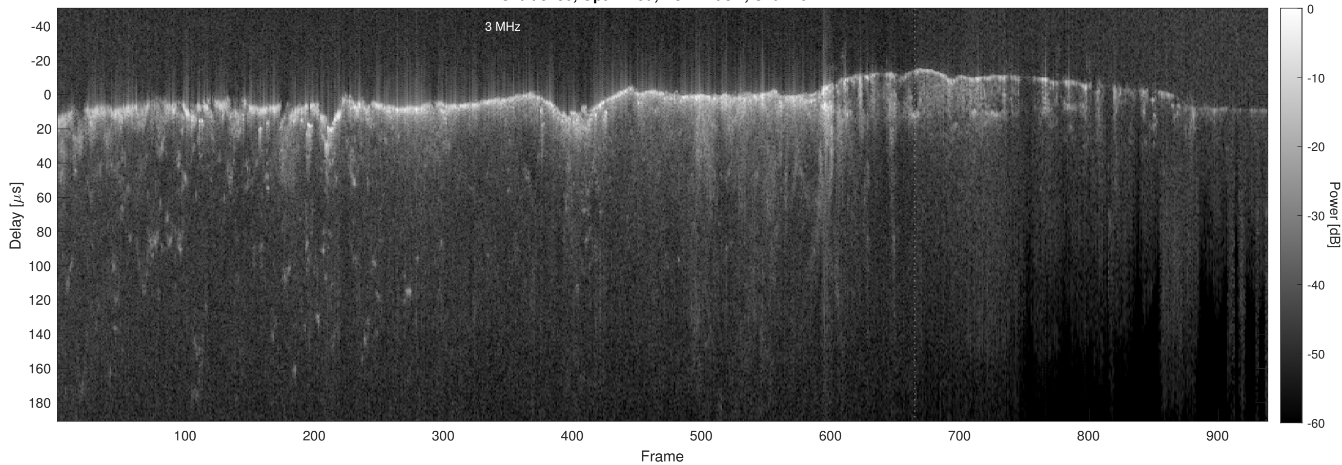
Orbit 8780, Optimized, No Window, Channel 2
