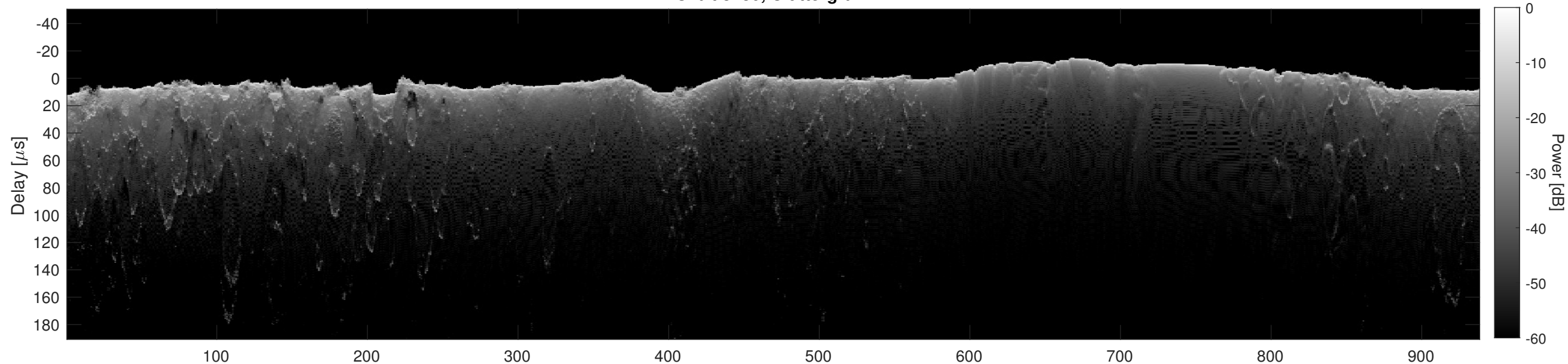
Orbit 8780, Cluttergram
