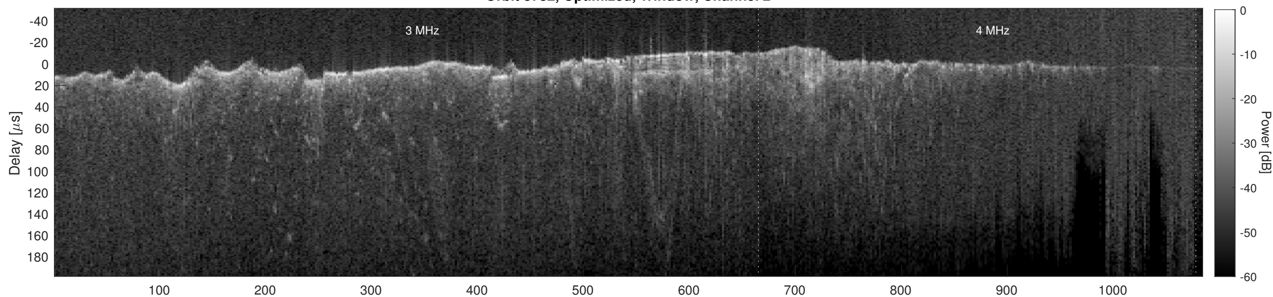
Orbit 8782, Cluttergram
